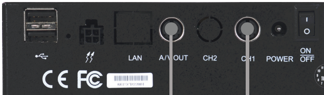
MDVR80 back panel
