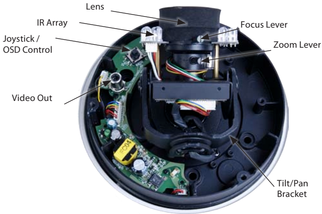
Internal Components - Cameras With IR
