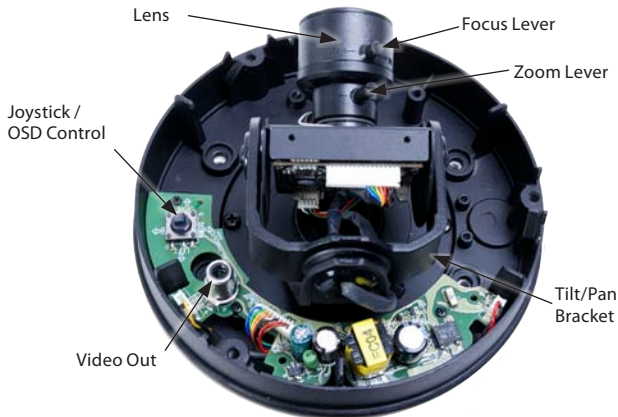
Internal Components - Cameras Without IR Array
